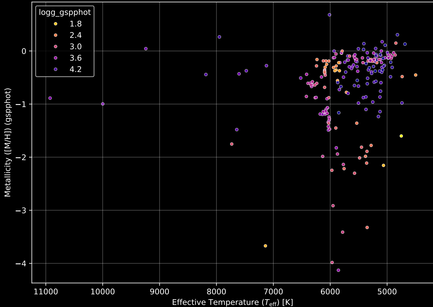
APOGEE DR17 Field: [N6397] Stellar Population Parameters (n= 210)
