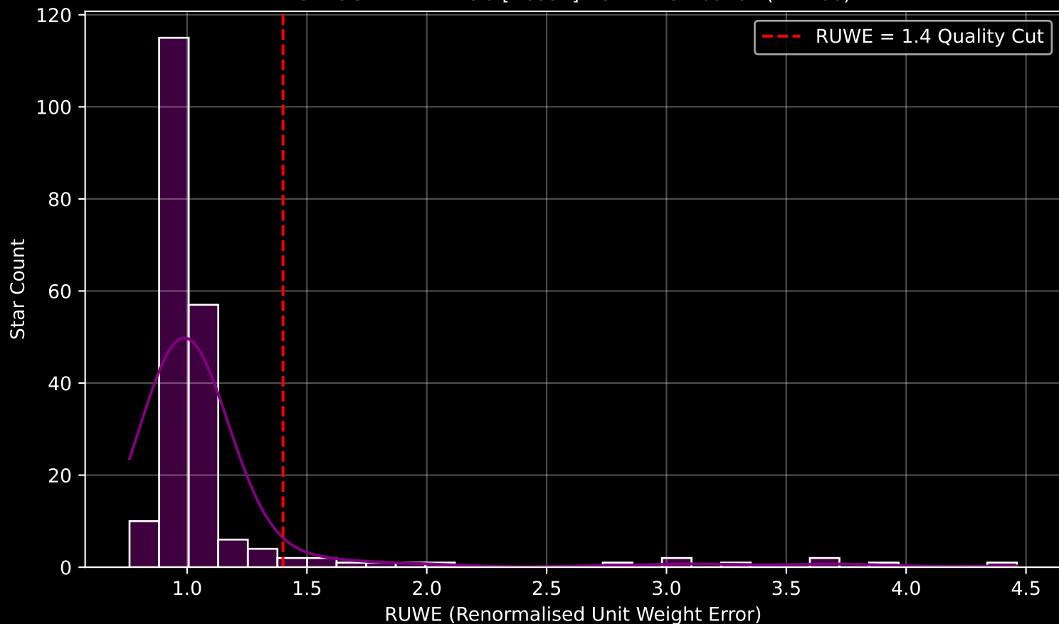
GAPOGEE DR17 Field [N6397] RUWE Distribution (n= 208)
