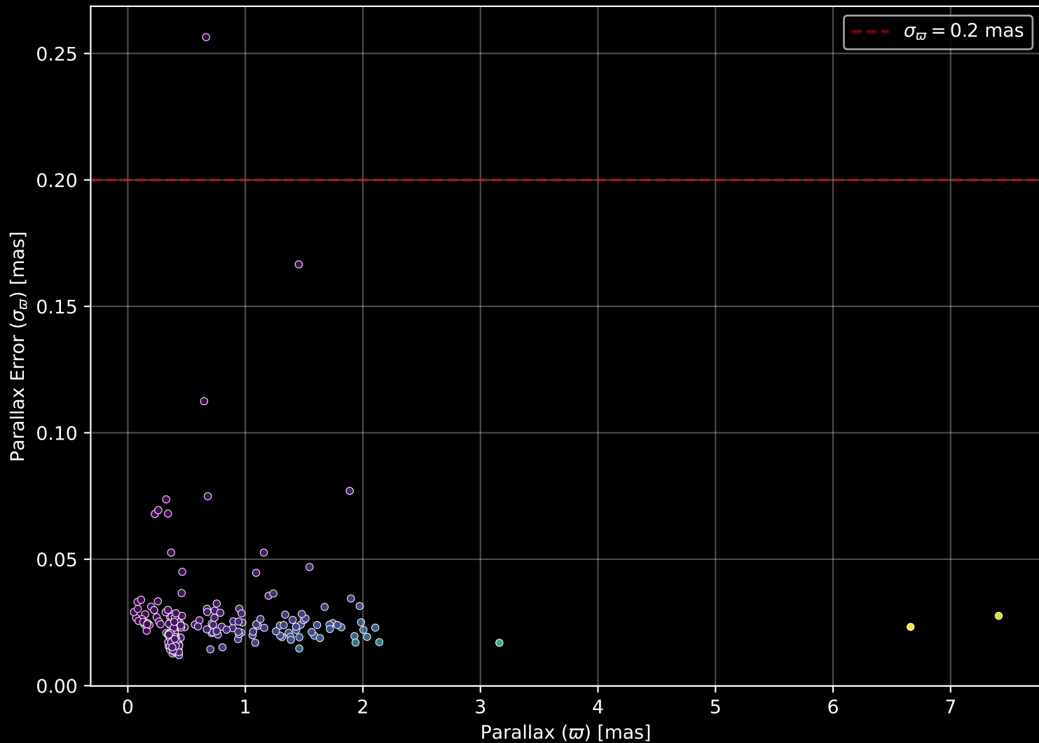
APOGEE DR17 Field: [N6397] Parallax Quality (n= 210)
