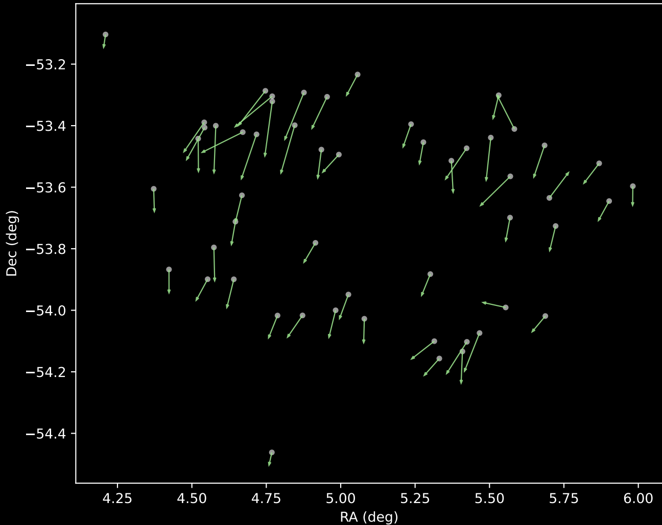
APOGEE DR17 Cluster 5 Proper Motion Vectors (n=53)
