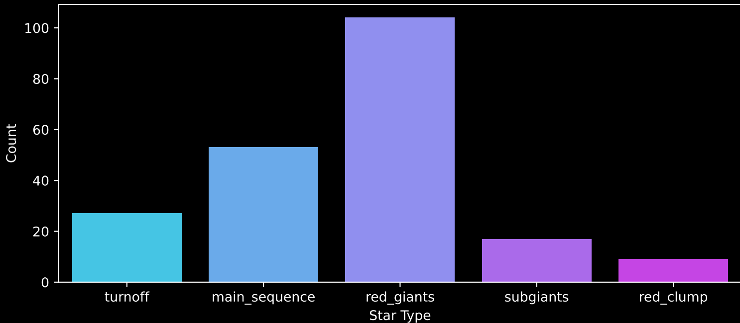
APOGEE DR17 Field: [N6397] Count plot of Star Type
