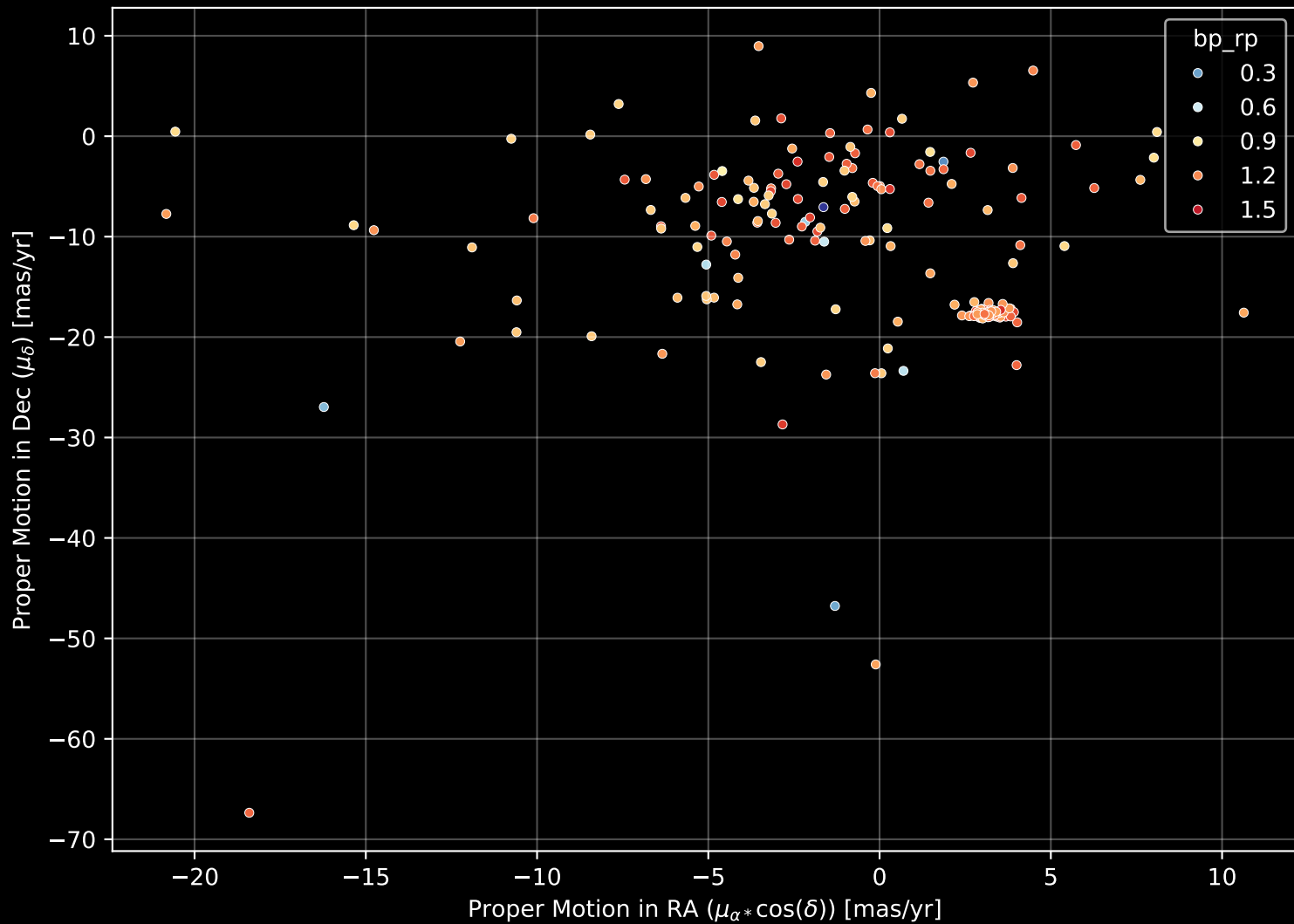
APOGEE DR17 Field: [N6397] Proper Motion Diagram (n= 210)
